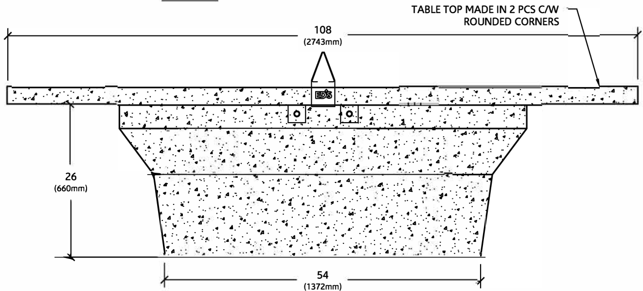
SIDE VIEW
